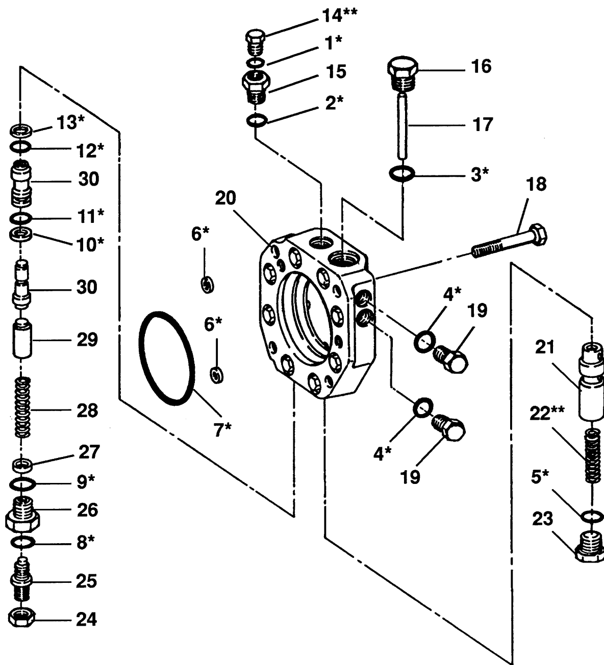
PUMP STROKE VALVE ASSEMBLY
